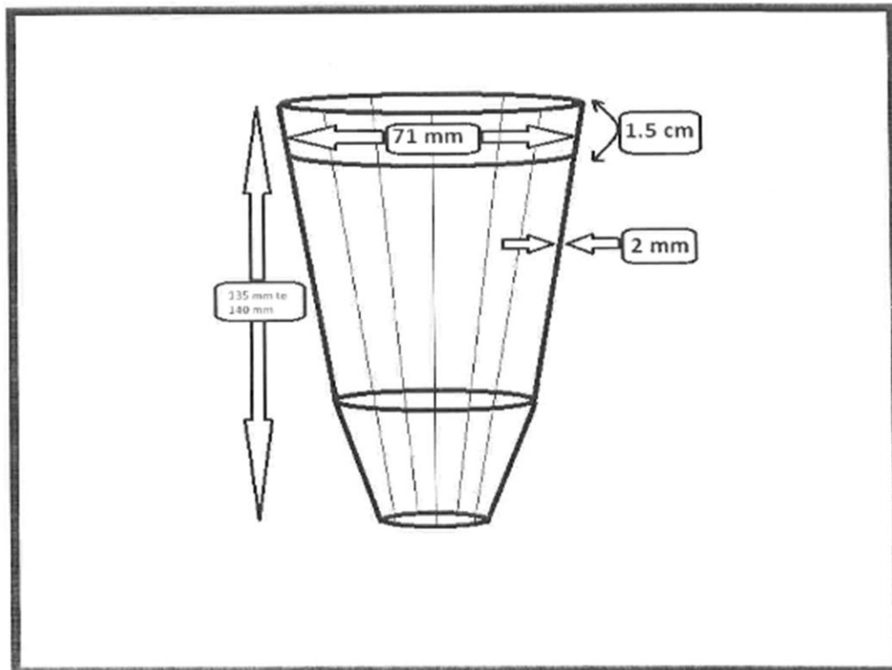
DRAWING OF ROOT TRAINER (VOLUME: 300 C.C.)
