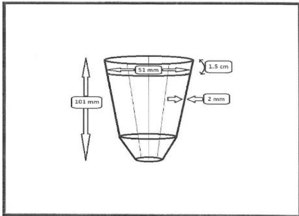
DRAWING OF ROOT TRAINER (VOLUME: 150 C.C. )
